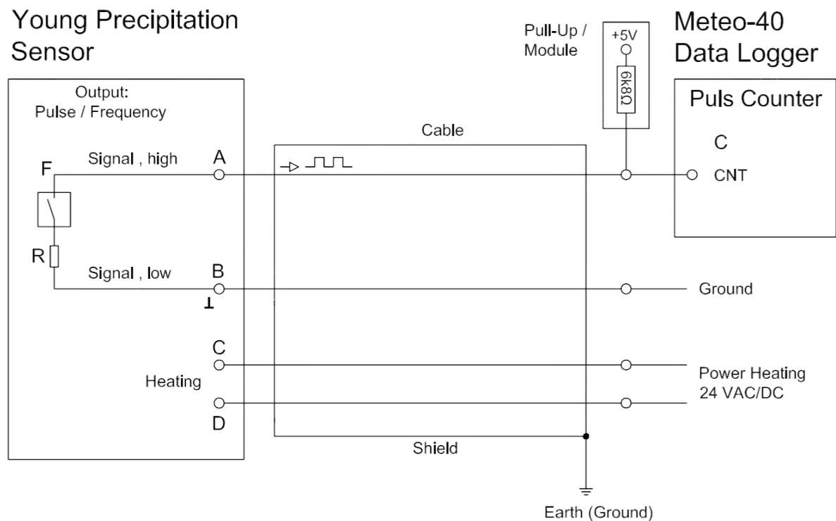
Sensor connection diagram to Ammonit Meteo-40 Data Logger
